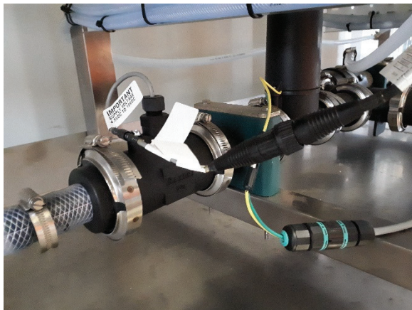
2.2 Flow Meter & Control Valve
