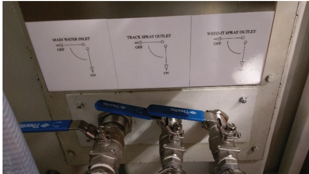
2.6 Track Spray Isolator (Centre)
