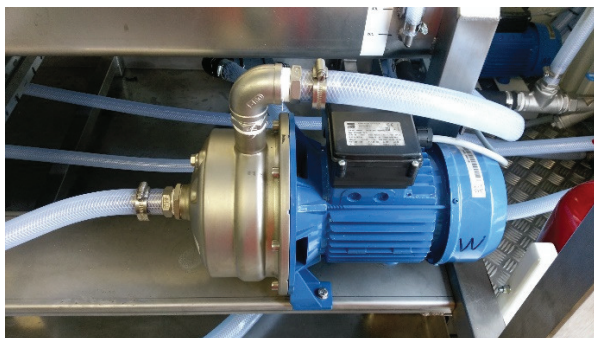
3.3 Weed-It Pump
